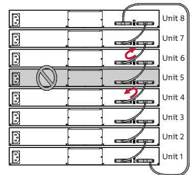
Figure 2. In the unlikely event of a switch failure, the stack integrity is maintained: cascade signals loop back at point of failure.
